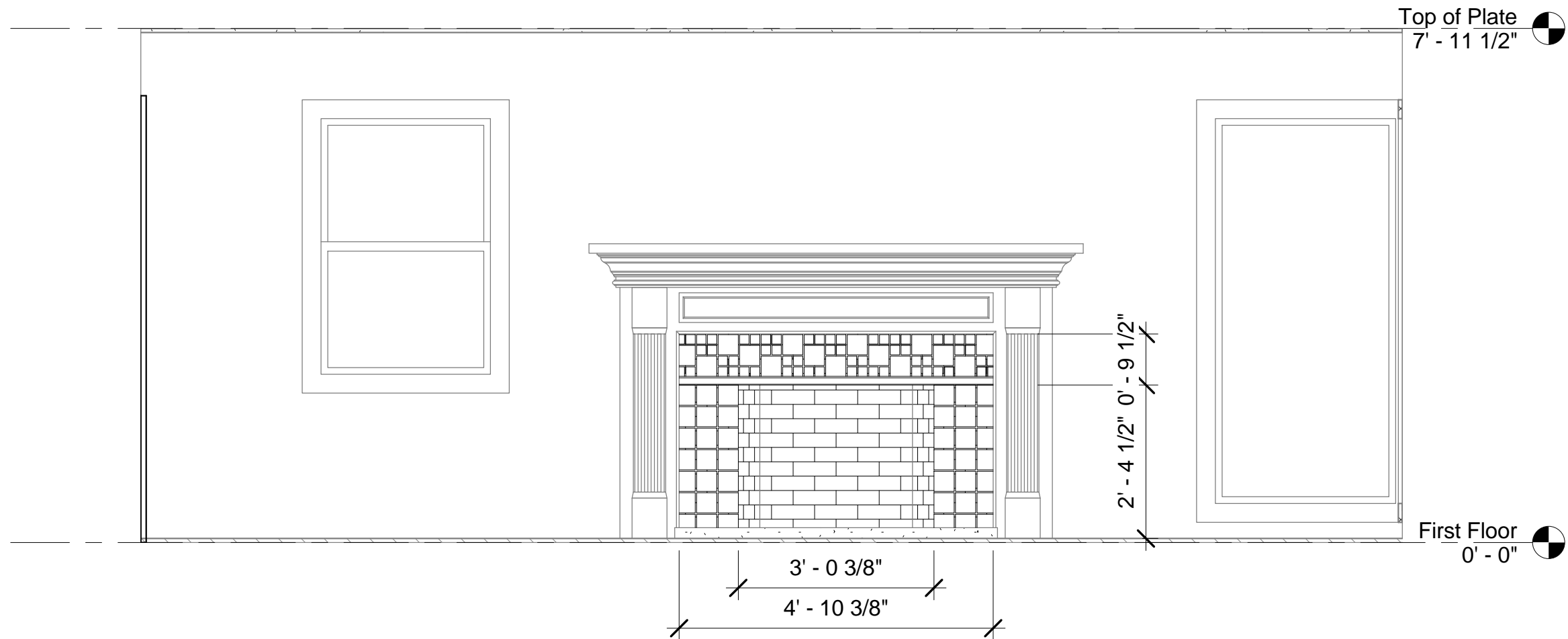
1 Fireplace Elevation 1/2" = 1'-0"
